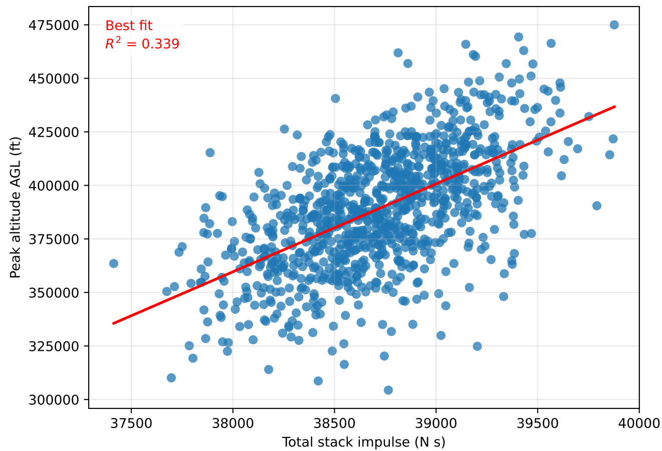
Stage impulse and mass sensitivity of apogee
